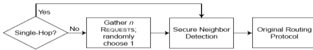
Figure 5: Combined Mechanisms to Secure MANET against Rushing Attacks
